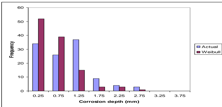
Figure 8: Comparison of predicted depth data to actual data for vessel age of 18-18.5 years old (RMSE of \pm 11.3 )
